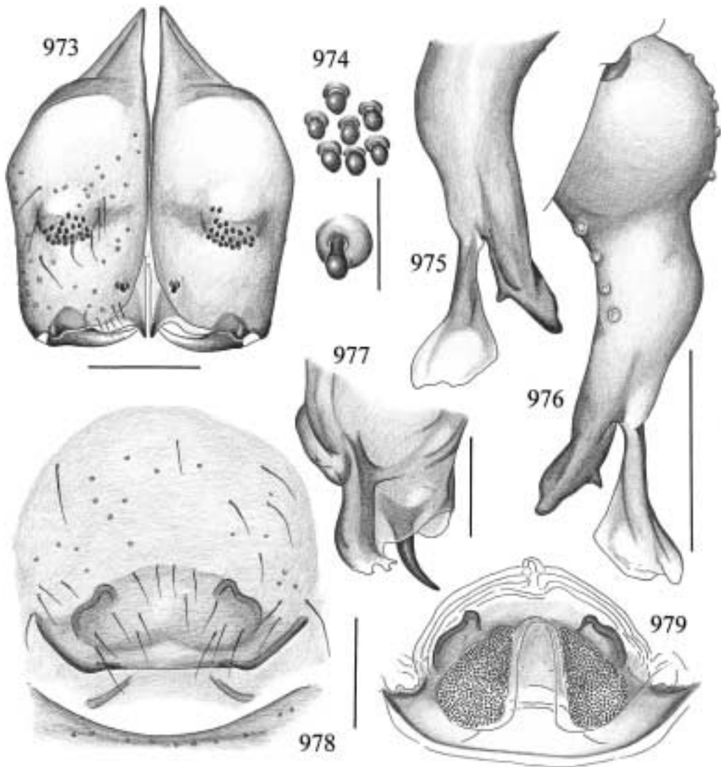
Figs. 973–979. Carapoia genitalis (Moenkhaus). 973 . Male chelicerae, frontal view. 974 . Modified hairs on male chelicerae. 975 . Right procurrus, prolateral view. 976 . Right procurrus, retrolateral view. 977 . Embolar division of right bulb, ~ prolateral view. 978 . Epigynum, ventral view. 979 . Epigynum, dorsal view. Scale lines: 0.2 mm (973, 975–979), 0.05 mm (974).
