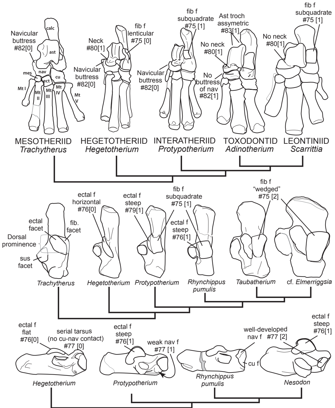
FIGURE 12. Hypothetical pedal transition series in Notoungulata showing left pes in dorsal view (upper row), left calcaneum in dorsal view (middle row), and left calcaneum in medial view (lower row). Illustrations are not to scale. Abbreviations are as follows: ast, astragalus; calc, calcaneum; cu, cuboid; ect, ectocuneiform; f, facet; fib, fibula; Mt, metatarsal; nav, navicular; sus, sustentacular; troch, trochlea.
