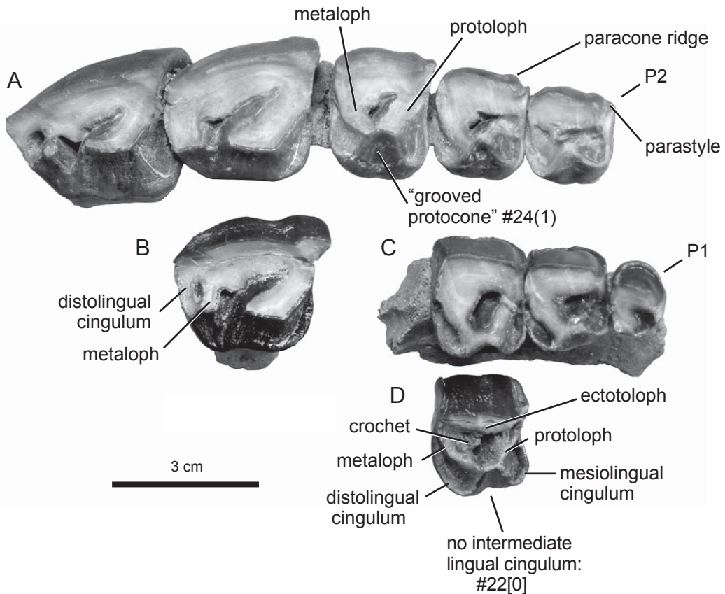
FIGURE 5. Upper cheek teeth of Elmeriglesia fieldia , new taxon. A , P 13386, holotype, P2–M2; B , PM 61102, right M1; C , PM 61101, right P1–P3; and D , P 15060, unworn, right P3. Scale bar applies to all.
