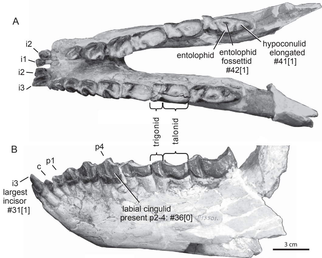
FIGURE 6. Mandible of Elmerriggsia fieldia (FMNH P 13501) in occlusal (A) and lateral (B) views.
