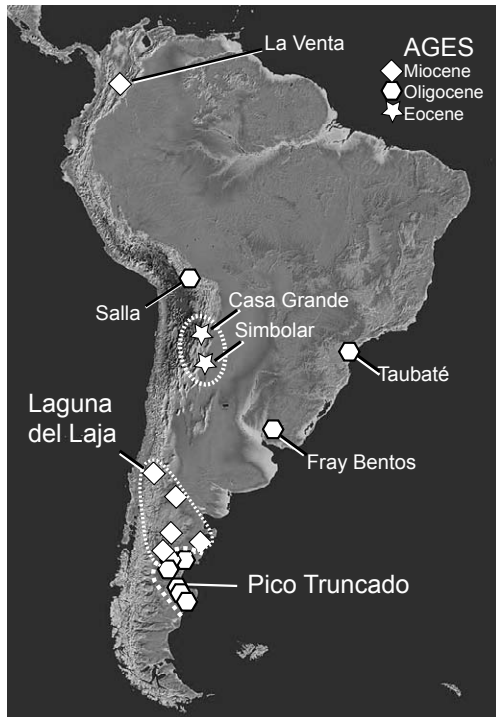
FIGURE 1. Geographic setting of leontiniid localities (background map adapted from NASA image).
