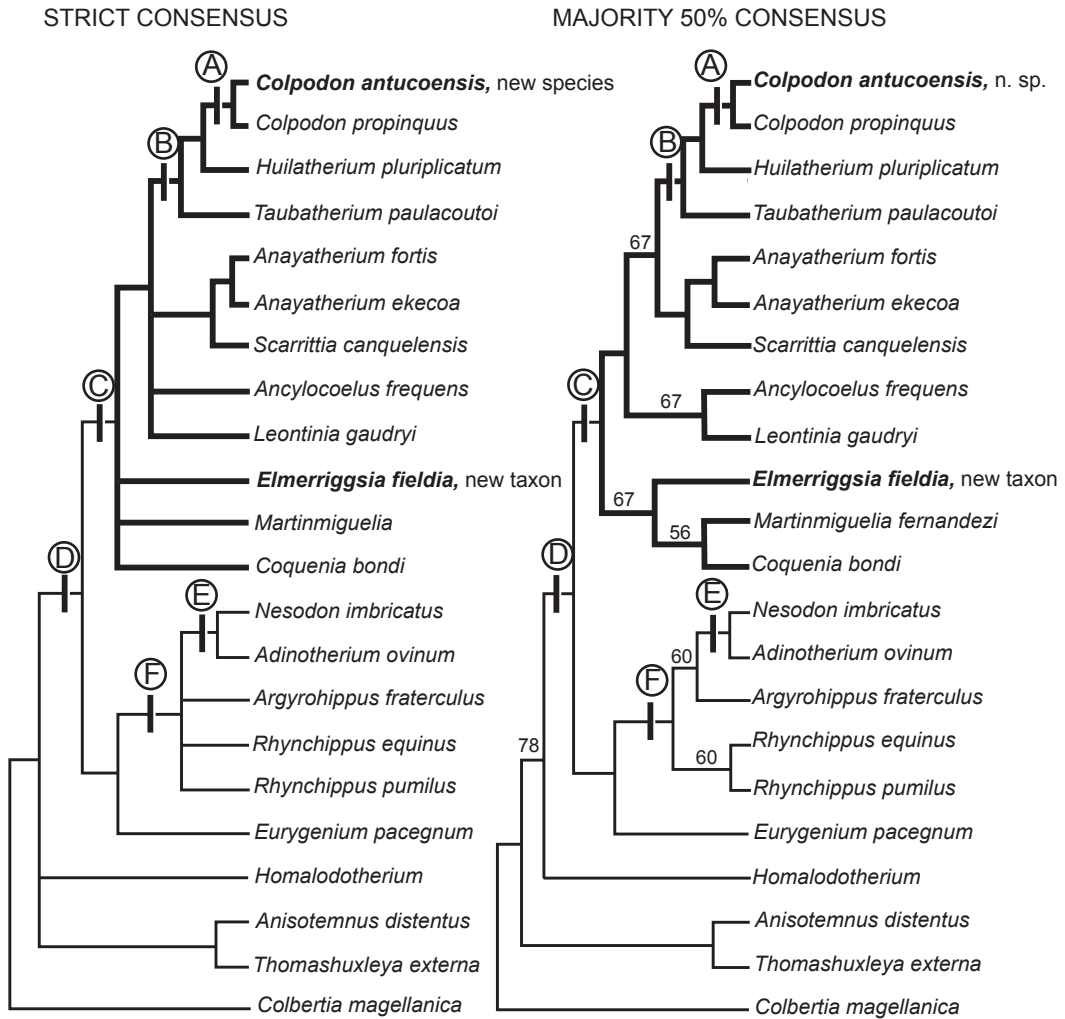
FIGURE 13. Cladogram of the “Toxodont” analysis. Strict consensus (left) and majority 50% consensus of the “Toxodont” phylogenetic analysis. Nodes: A, Colpodon ; B, “Tropical clade”; C, Leontiniidae; D, “advanced Toxodontia”; E, Toxodontidae; F, “notohippid” + Toxodontidae. Numbers at nodes represent percent support when support is less than 100%.
