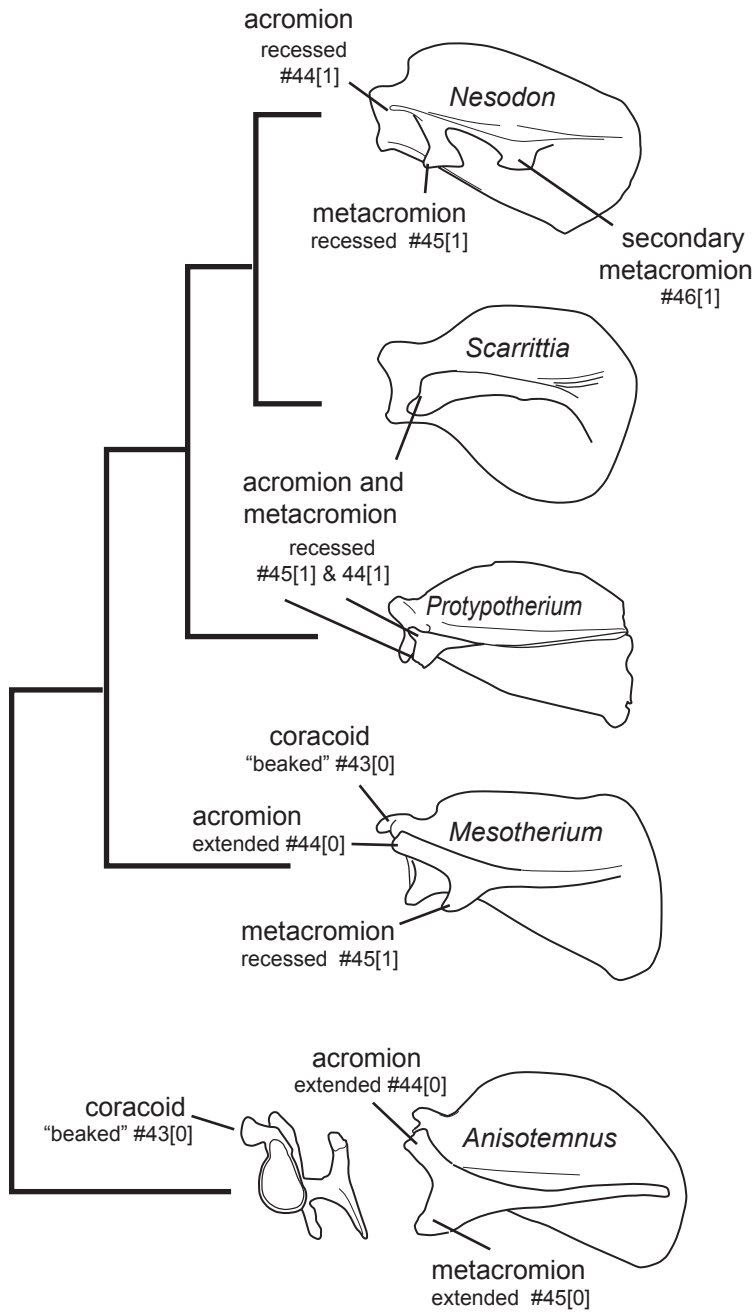
FIGURE 10. Hypothetical scapular transition series in Notoungulata. Not drawn to scale.
