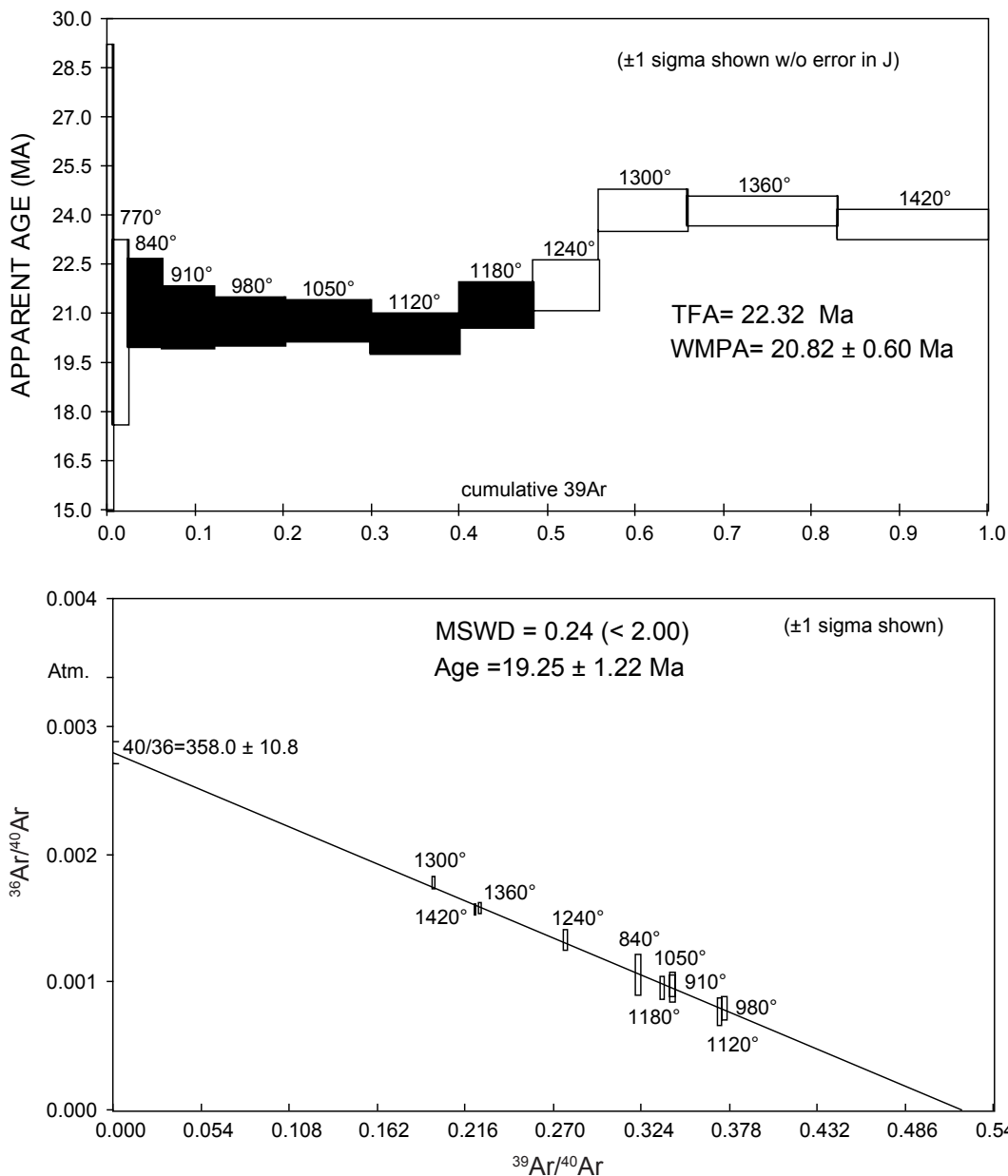
FIGURE 4. ^{40}\text{Ar}/^{39}\text{Ar} age spectra and inverse isochron plots for samples CH-31 (above) and CH-32 (opposite page). Age spectra illustrate apparent age versus cumulative fraction of ^{39}\text{Ar} released. Shaded boxes indicate steps used to calculate weighted mean plateau ages. Plotting these steps suggests that most of them fall on simple isochrons with a ^{40}\text{Ar}/^{36}\text{Ar} ratio of the trapped component somewhat higher than atmospheric gas, giving a more reliable estimate of the ages at ~19.5 Ma, or ~19.8 Ma when corrected for a revised age of the Fish Canyon Tuff standard.
