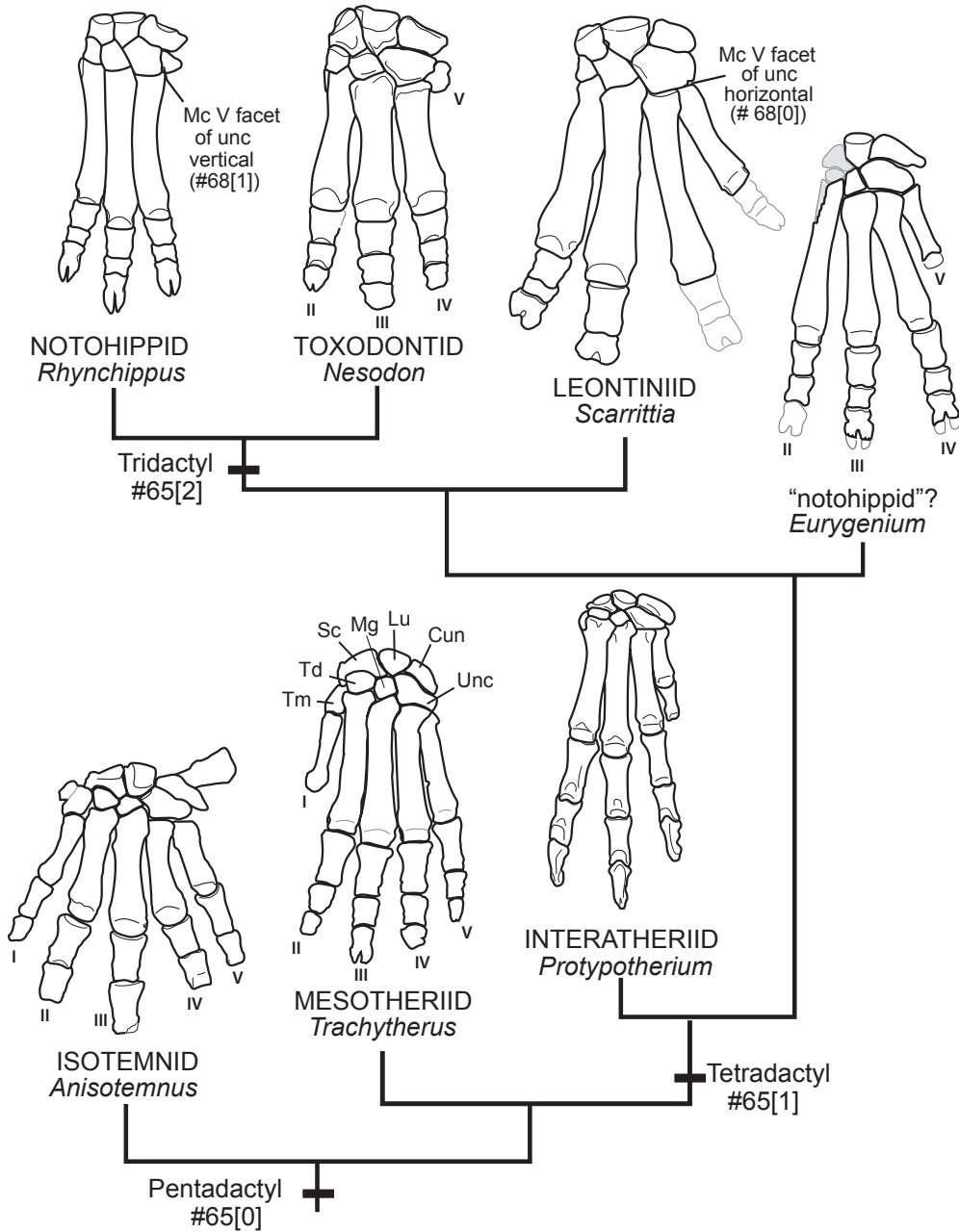
FIGURE 11. Hypothetical manual transition series in Notoungulata. All hands shown as left. Not drawn to scale. Abbreviations: Cun, cuneiform; Lu, lunate; Mg, magnum; Sc, scaphoid; Td, trapezoid; Tm, trapezium. Roman numerals indicate digit number.
