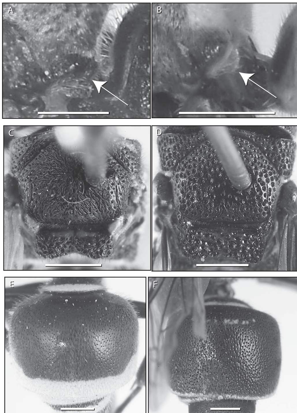
FIGURE 9. (A) B. albula and (B) B. propodealis , propodeal valve in lateral view; (C) B. moebiana and (D) B. albula , scutum in dorsal view; (E) B. moebiana and (F) B. albula , metasomal tergum II in dorsal view. Scale bars = 1.0 mm.
