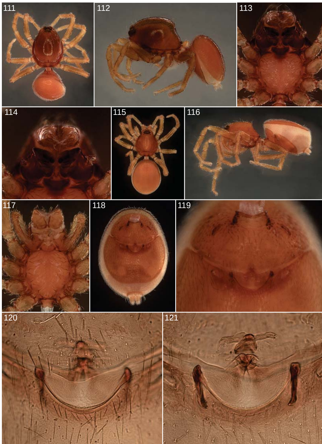
FIGURES 111–121. Hexapopha osa , new species, male (111–114) and female (115–121). 111, 115. Habitus, dorsal view. 112, 116. Same, lateral view. 113, 117. Sternum, ventral view. 114. Endites, same. 118. Abdomen, same. 119, 120. Genitalia, same. 121. Same, dorsal view.
