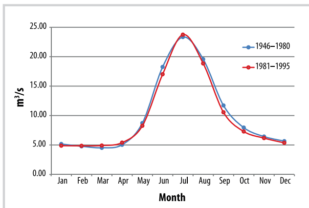
FIGURE 6 Changes in monthly Khojobakirgan river flow. (Graph based on data from Rysbekov 2008)
