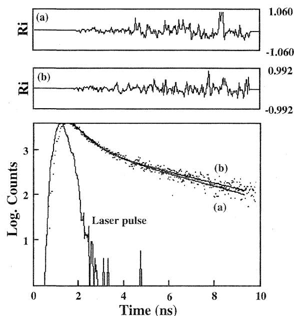
Fig. 3. Fluorescence decay curves from the wings of M. sulkowskyi monitored at 510 nm (curve a) and at 560 nm (curve b). Excitation wavelength was 337.1 nm. The upper frames show the residual (Ri) plots.
