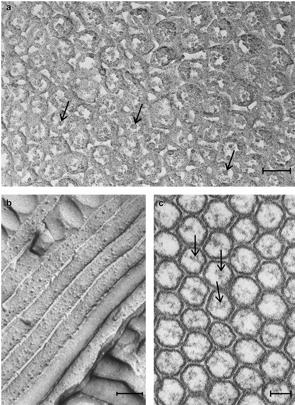
Fig. 14. (a): Deep-etched crayfish rhabdom, showing microvilli in transverse section and core filaments (arrows). Scale=0.1 \mu m. (Courtesy of E. Eguchi). (b): Freeze-fractured crayfish rhabdom, showing photopigment molecules in microvillar membranes. Scale=0.1 \mu m (after Meyer-Rochow and Eguchi 1984). (c): High power electron micrograph of transversely sectioned microvilli from the dark adapted crayfish eye, showing core filament (arrows). Scale=50 nm.
