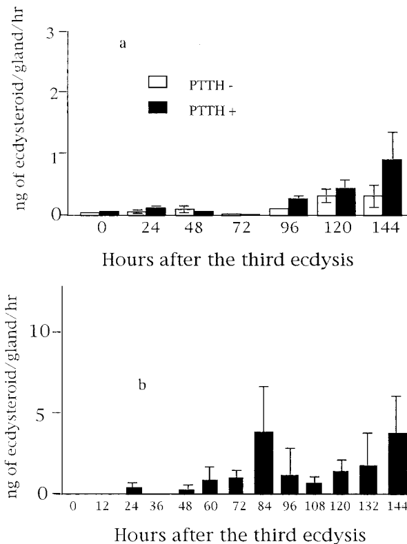
Fig. 5. (a) PG responsiveness to PTTH of the recessive trimolter E7 strain in the fourth larval instar. The experimental methods and representation of data are described in Fig. 4 (a).
