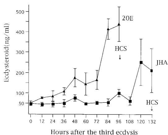
Fig. 3. Hemolymph ecdysteroid titer (ng/ml) of the hormone-treated trimolter E7 strain of Bombyx mori after the third larval ecdysis: —○, larvae fed mulberry leaves treated with 20E (20ppm) from the third ecdysis to 72 hr after the third larval ecdysis; —■, larvae treated with JHA by topical application. JHA (2 µg/larva) was applied on the back of the insects at 24 hr after the third ecdysis. RIA was carried out using 20E as a standard compound. Each datum represents the mean and SEM of 3–4 insects. HCS indicates the timing of head-capsule slippage.
