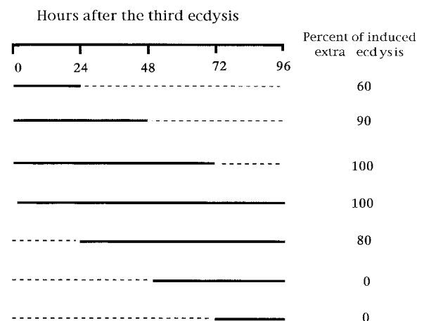
Fig. 2. Effects of 20E feeding time on the induction of the extra larval ecdysis of the trimolter. Solid lines indicate the period of feeding with mulberry leaves treated with 20E (20ppm). Dotted lines indicate the period of feeding with mulberry leaves without 20E. Numbers on the right of each schedule indicate the percent of induced extra larval ecdysis (n=10).
