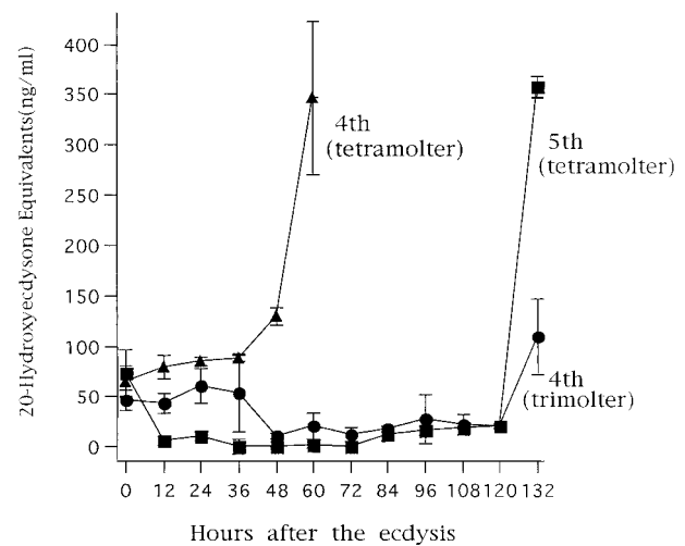
Fig. 1. Hemolymph ecdysteroid titer (ng/ml) after the third larval ecdysis of the trimolter E7 strain (—) and after the third (—) and the fourth (—) larval ecdysis of the tetramolter of Bombyx mori . RIA was carried out using 20E as a standard compound. Each datum point represents the mean and SEM of 3–4 insects.
