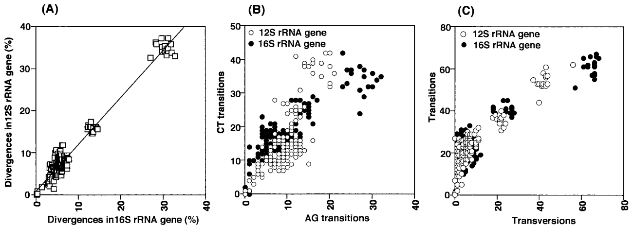
Fig. 5. (A) Dependence of percent sequence divergences of the 12S rRNA gene on the 16S rRNA gene. (B) Dependence of C↔T (CT) transitions on A↔G (AG) transitions of the 12S and 16S rRNA genes. (C) Dependence of transitions on transversions of the 12S and 16S rRNA genes.
