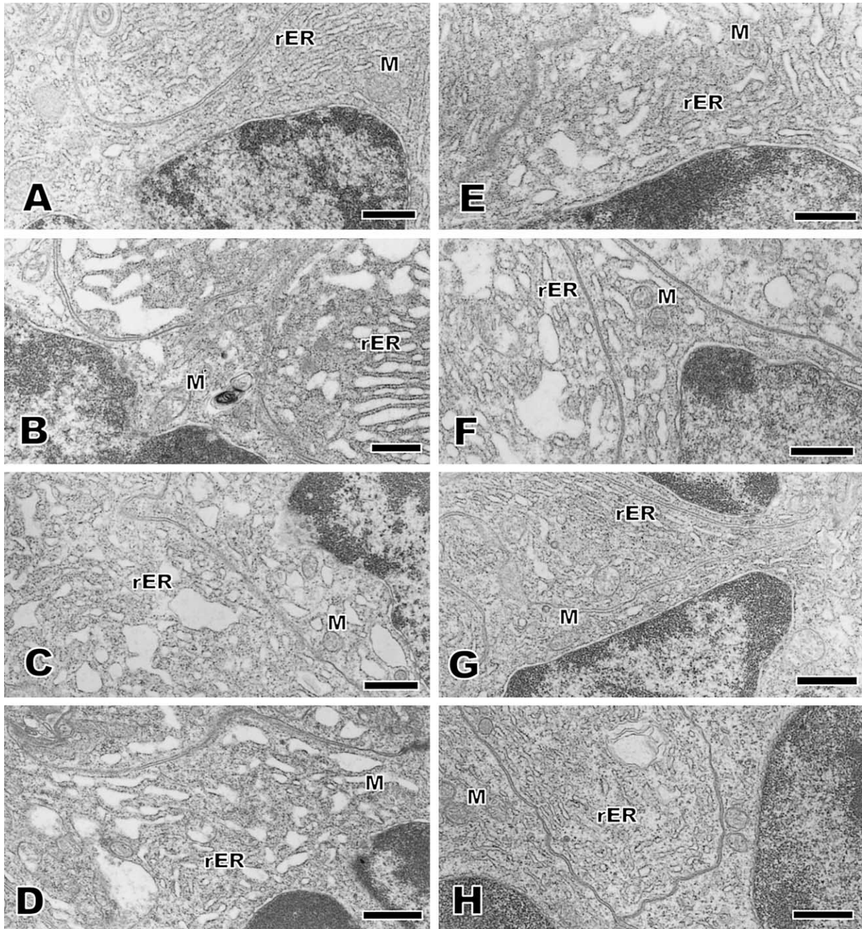
Fig. 7. Androgenic gland structure during the molt cycle in Macrobrachium rosenbergii . A, orange-claw male at molt stage A; B, orange-claw male at stage C; C, orange-claw male at stage D 1 ; D, orange-claw male at stage D 2 ; E, small male at stage B; F, small male at stage C; G, small male at stage D 1 ; H, small male at stage D 2 . M, mitochondria; rER, rough endoplasmic reticulum. Bar=1 \mu m.
