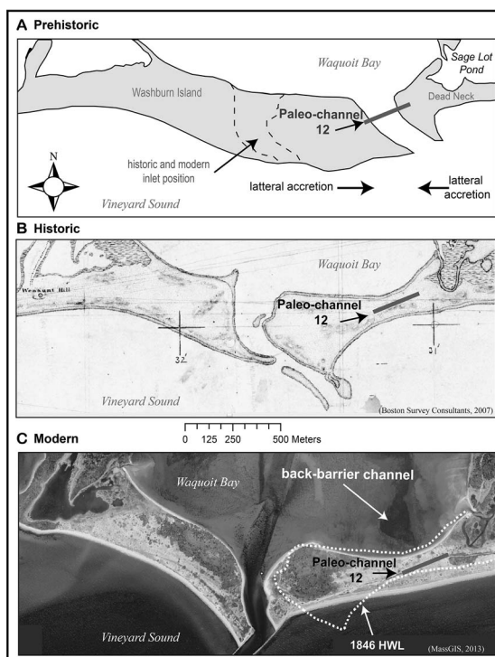
Figure 10. Morphologic evolution of the Waquoit barrier in the vicinity of Dead Neck and Washburn Island. (A) Conceptual model of prehistoric configuration with interpreted main channel location based on position of Paleochannel 12 shown with dark gray line. The general location of both the modern and historic inlet is shown with the white dashed line. Horizontal arrows indicate the lateral migration and infilling of the former inlet. (B) 1846 Coast Survey map with position of Paleochannel 12 shown with black line (Boston Survey Consultants, 2007). (C) A 2011 orthophotograph with current barrier configuration. The 1846 high water line (HWL) is shown with the white dashed line. The position of Paleochannel 12 is identified with a black line adjacent to a back-barrier channel feature interpreted to be a surficial indicator of the prehistoric inlet.
