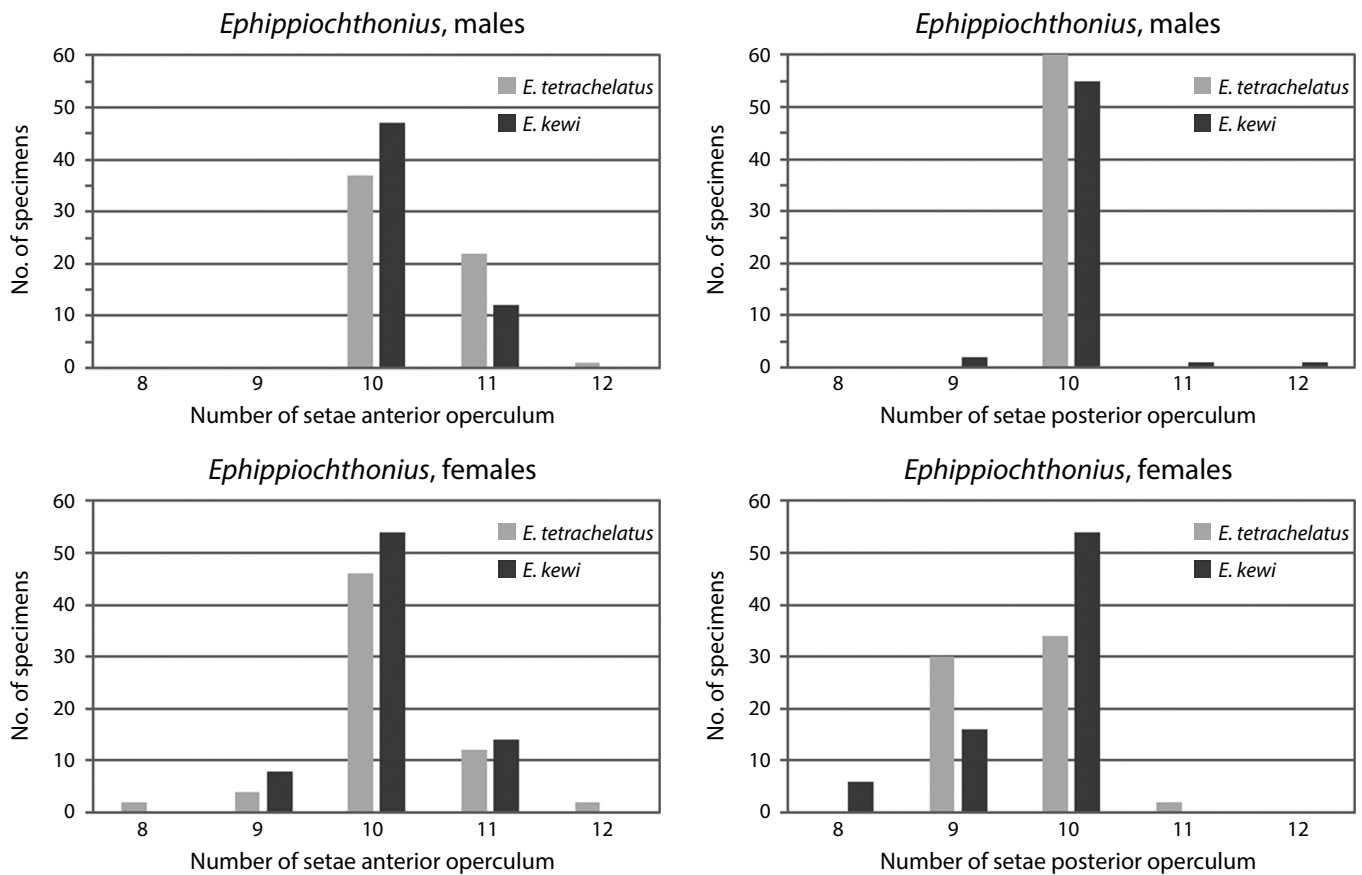
Fig. 5: Frequency diagrams of different setae number on anterior and posterior genital opercula for both males and females of Ephippiochthonius kewi Gabbutt, 1966 and E. tetrachelatus (Preysslser, 1790)
