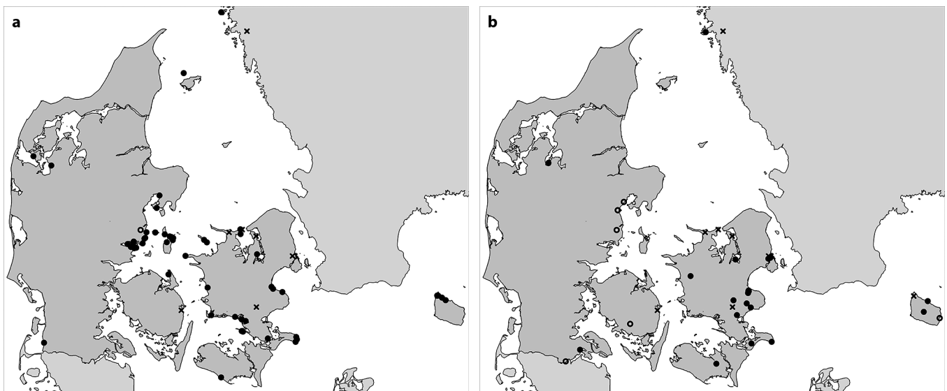
Fig. 2: Distribution of Ephippiochthonius species. a. Ephippiochthonius kewi Gabbutt, 1966; b. Ephippiochthonius tetrachelatus (Preysslner, 1790). ● = specimens found in natural habitats; ○ = specimens found in greenhouses, railways and harbour wastelands; × = assumed hybrids of E. kewi and E. tetrachelatus
