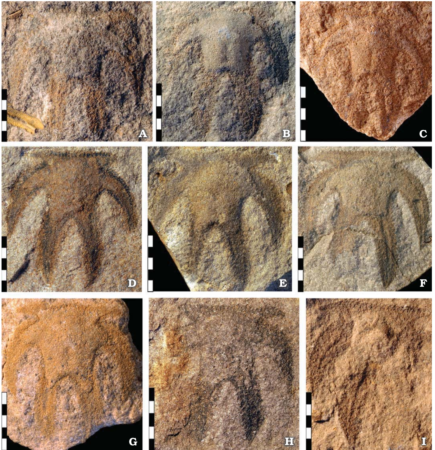
Fig. 2. The marrellomorph arthropod Furca bohémica Fritsch, 1908 from the Upper Ordovician (Sandbian) of Bohemia (Ostrý Hill and Veselá, Beroun District). A. NML 32991. B. NML 32992. C. NML 32993. D. NML 32994a. E. NML 32994b. F. NML 32995. G. NML 32996. H. NML 32997. I. NML 33000. Scale bars 10 mm.
