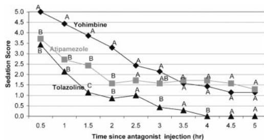
FIGURE 1. Mean sedation scores for 21 captive white-tailed deer immobilized with tiletamine-zolazepam/xylazine (220 mg tiletamine-zolazepam [ 4.5 \pm 0.4 mg/kg] and 110 mg of xylazine [ 2.2 \pm 0.2 mg/kg]) and given one of three \alpha_2 antagonists, October to November 2002, Athens, Georgia. Antagonist treatments with the same letter at each time point are not significantly different. Sedation score of 5 = lateral recumbency with no sign of reversal. Sedation score of 0 = no sign of sedation.
