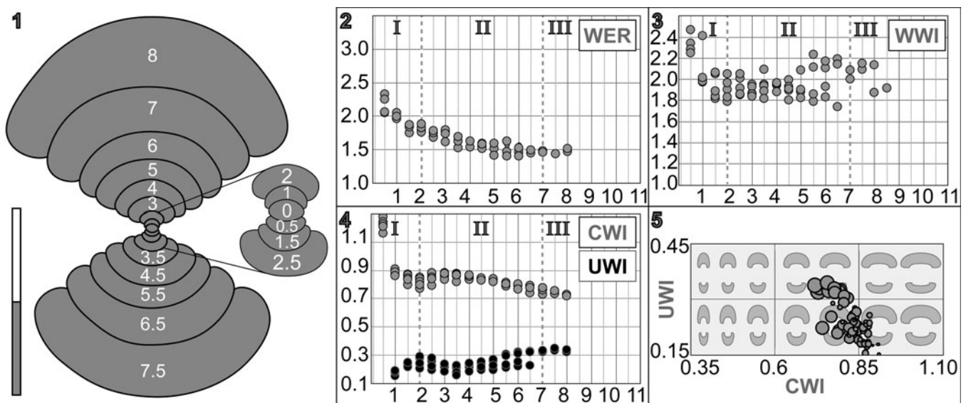
Figure 13. Ontogenetic analysis of Ptychites embreei n. sp. (1) Cross section of specimen GSUB C9642, scale bar units 5 mm. (2–4): Ontogenetic development of the whorl expansion rate ( WER_n = (dm_n/dm_{n-0.5})^2 ), whorl width index ( WWI_n = ww_n/wh_n ), umbilical width index ( UWI_n = uw_n/dm_n ) and the conch width index ( CWI_n = ww_n/dm_n ) plotted against number of half whorls (ontogenetic stages). (5) Ratio between UWI and CWI of the available specimens. Bubble size refers to number of half whorl; the picture in the background shows the shape of the last complete whorl (developed by Korn, 2010). Roman numbers refer to interpretation of different life phases; I: Hatchling, II: Juvenile, III: Subadult–adult; for more detailed explanations see Walton and Korn (2017).
