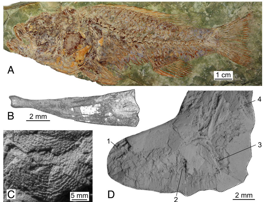
FIGURE 13. † Rebekkachromis ngororus from the Rebekka site, OCO-3-3a. A , complete skeleton of the holotype; B , urohyal, reversed; C , imbricate cycloid scales, anterior on top; D , preopercle, in lateral view. C and D are coated with ammonium chloride. Numbers denote the sensory canal pores of the preopercle, dotted lines denote a fracture and the outline is uncertain.
