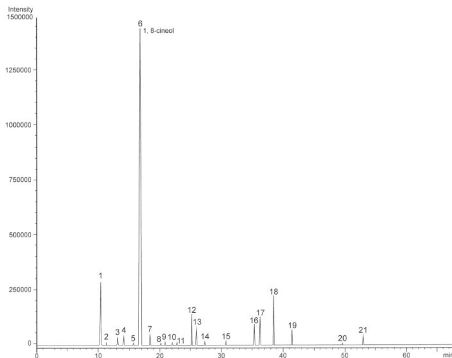
Fig. 1. GC chromatogram of rhizomes of A. galanga essential oil.
