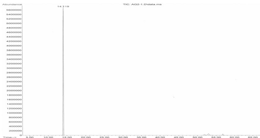
Fig. 2. Chromatogram of positive active compound from A. galanga after TLC.
