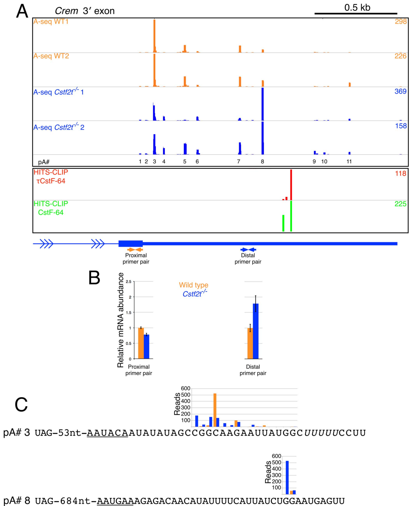
FIG. 2. Crem cleavage/polyadenylation sites change in wild-type and Cstf2 -/- seminiferous tubules. A ) A-seq reads representing cleavage/polyadenylation sites mapped on the mouse genome (mm10) from two wild-type (WT1, WT2, top orange bars) or two Cstf2 -/- ( Cstf2 -/- 1, Cstf2 -/- 2, middle blue bars) mice. Values in orange (wild type) and blue ( Cstf2 -/- ) on right represent the highest number of reads assigned to a specific 3' cleavage site in the corresponding tracks. Specific polyadenylation sites are designated 1 through 11 (pA#1–11, indicated at bottom). Bottom panels show \tau CstF-64 (red, top) and CstF-64 (green, bottom) binding sites determined using HITS-CLIP. The last intron and 3' exon of Crem are shown (blue). Distal and proximal
