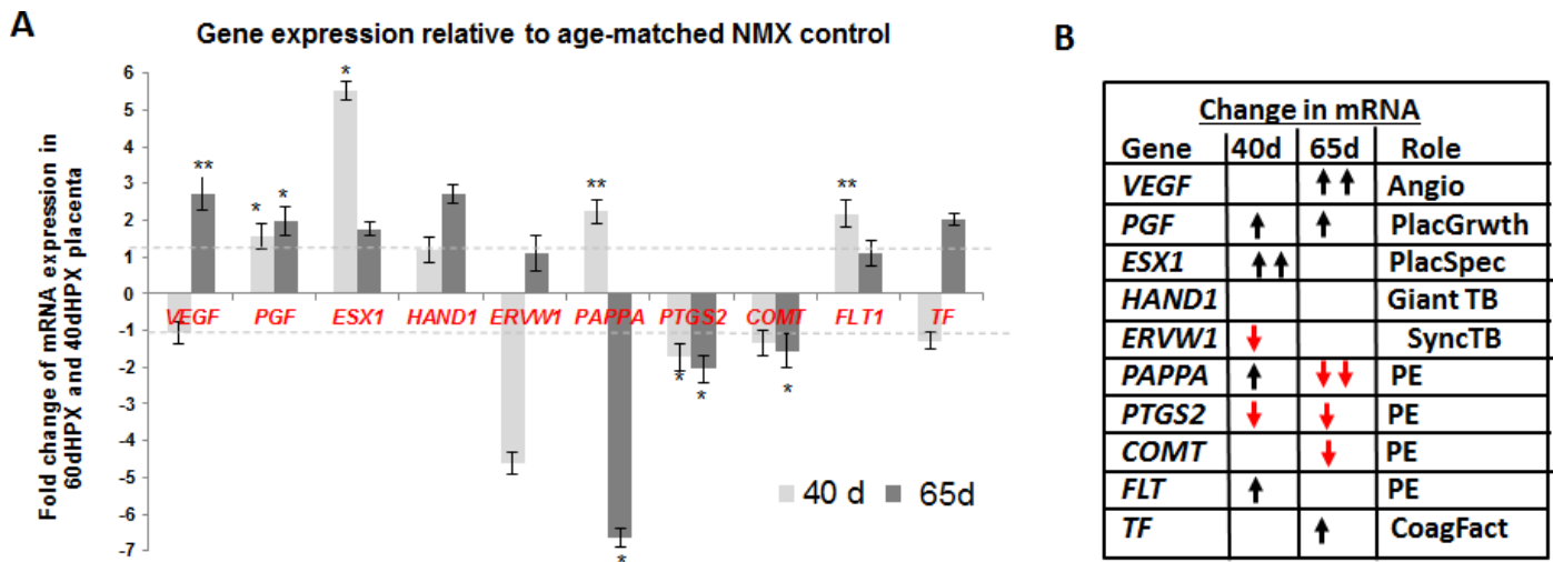
FIG. 5. Effects of hypoxia (HPX, 10.5% O 2 ; n = 6, 40 days; n = 6, 65 days) on placental mRNA expression relative to age-matched normoxic (NMX, n = 5 for each gestational age) controls. A Fold changes of placental specific gene expression caused by HPX compared to age match NMX controls at midterm (40 days, light gray bars) and term (65 days, dark gray bars) pregnancy are shown. Data are normalized to endogenous beta-actin and expressed relative to NMX. Dashed line indicates 1.4-fold change, single or double asterisk denotes statistical difference P < 0.05 or P < 0.01 from NMX control, respectively. B Table illustrates the directional changes (arrows) obtained from the gene expression data on the left along with identification of the role of each gene.
