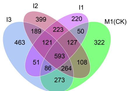
Fig. 2. A Venn diagram showing the number of shared operational taxonomic units across different soil samples from tea- Pleurotus intercropping: 1 yr tea-fungus intercropping plantations (I1), 2 yr tea-fungus intercropping plantations (I2), 5 yr tea-fungus intercropping plantations (I3), and 5 yr chemically fertilized monoculture plantations (M1). [Colour online.]
