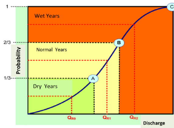
Figure 4. Class divisions based on the probability in the Markov model.
