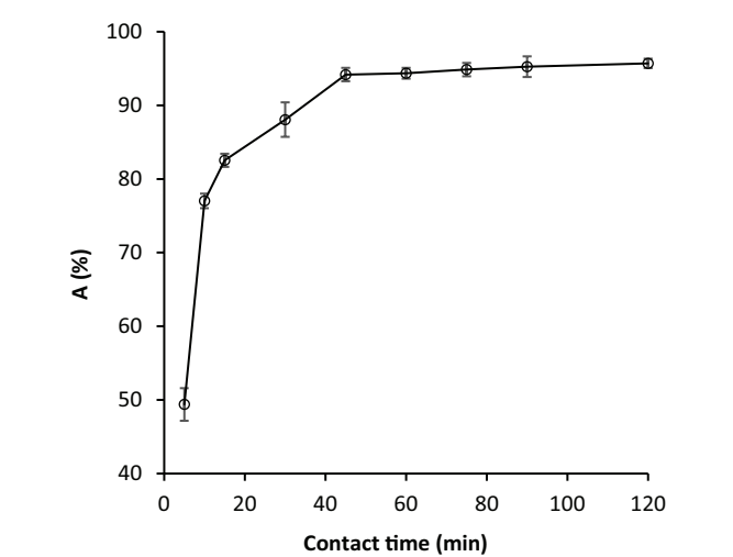
Figure 1. Effect of contact time on phosphate adsorption onto pumice.
