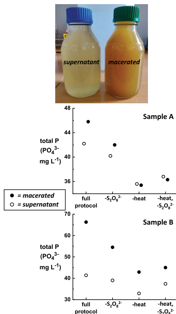
Figure 2. Comparison of total P results obtained during systematic omission of testing steps for two raw wastewater samples A and B collected from the Coimbatore field testing site. The photograph shows the typical appearance of the supernatant and macerated sample fractions. For each sample, both the macerated fraction (closed circles) and the supernatant fraction (open circles) were measured. The macerated fraction contains more fecal matter and thus a higher total P concentration. Omitting the heating step ("–heat") from the testing protocol has the largest effect on the measured total P concentration, while omitting the persulfate reagent ("– S_2O_8^{2-} ") has a smaller effect that is most visible for the macerated fraction. Samples were diluted with distilled water by 10\times to 25\times to bring them within the range of the total P Hach test kit.
