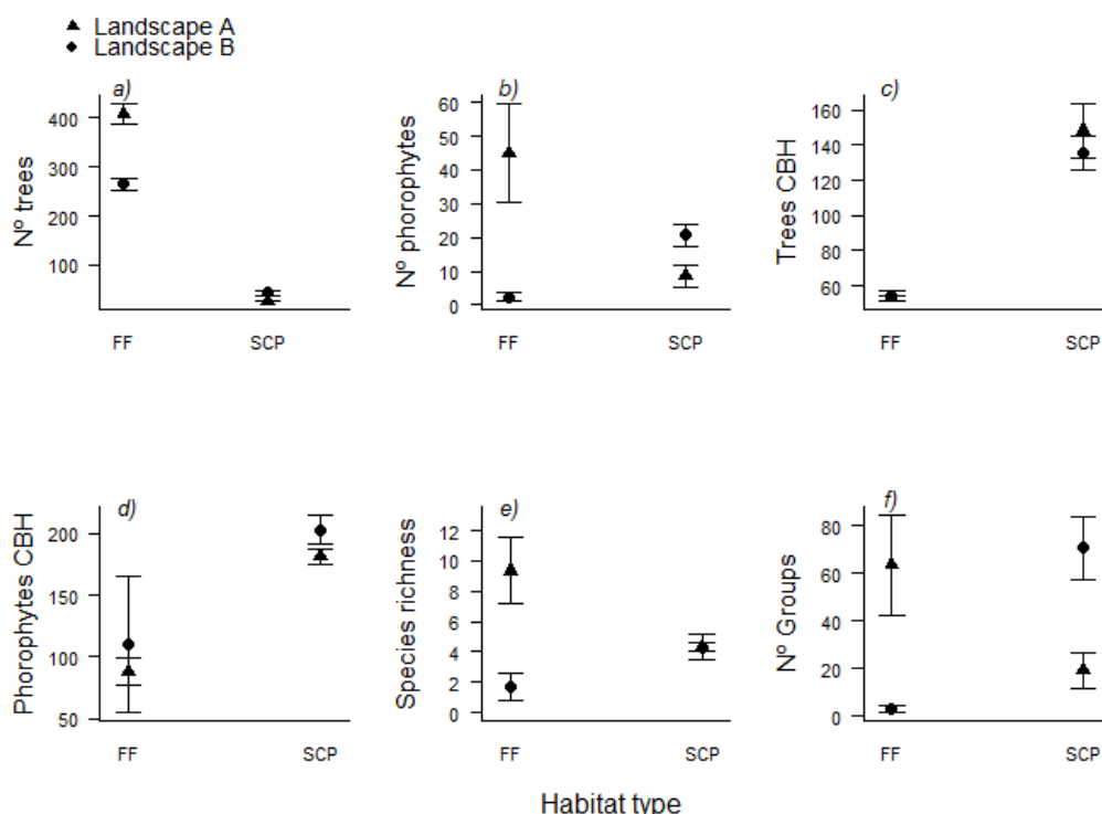
Fig.2. Comparisons between the mean number of trees (a) and phorophytes (b), mean CBH of trees (c) and phorophytes (d), and the mean number of species (e) and stands (f) of Aechmea and Hohenbergia in forest fragments (FF) and shade cocoa plantations (SCP) in landscape A and B. Vertical bars represent the standard error.
