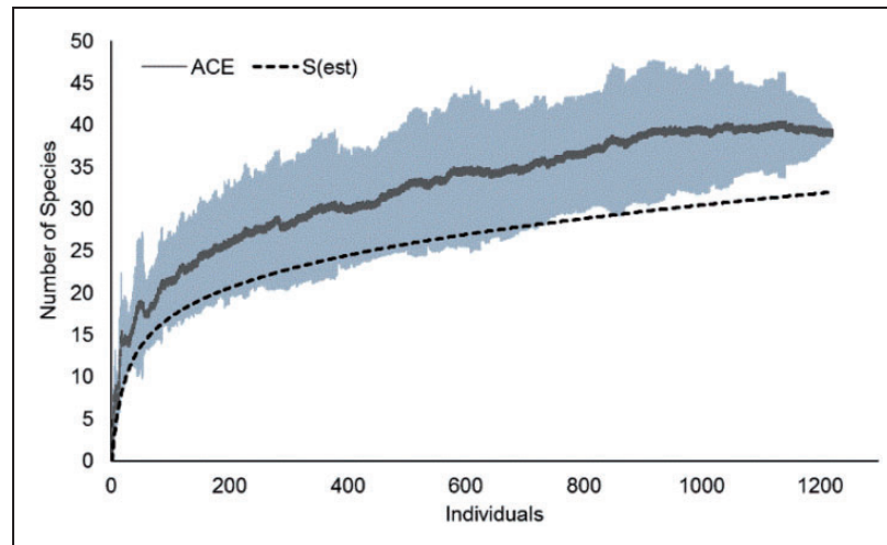
Figure 2. Expected number of species ( S(est) ; dashed line) and mean ( \pm SD ) abundance coverage-based estimator of species richness (ACE; solid line) for snakes detected during road-kill surveys conducted on both the primary road and secondary roads in the municipalities of Pampa Grande, Mairana, and Samaipata, Florida Province, Santa Cruz Department, Bolivia.
