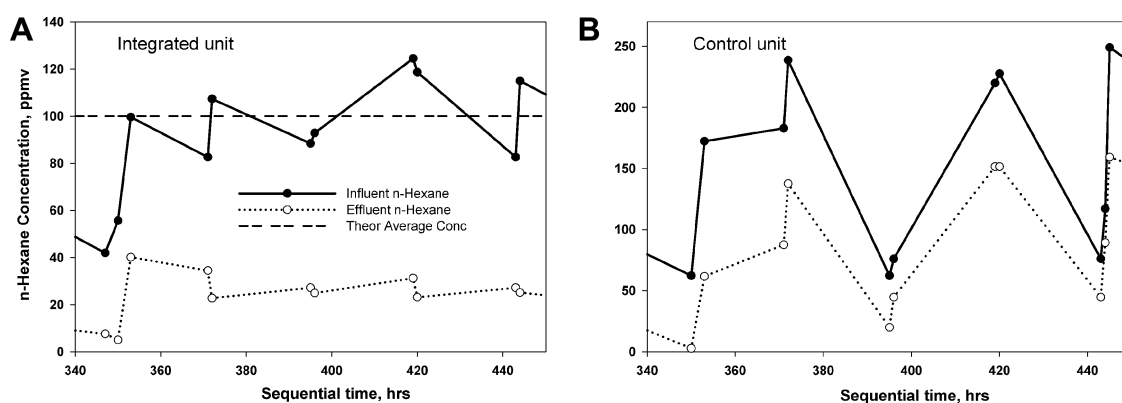
Figure 3. Removal performances of integrated unit and control unit with time after starvation: data presented for few hours after starting up the TBAB.
