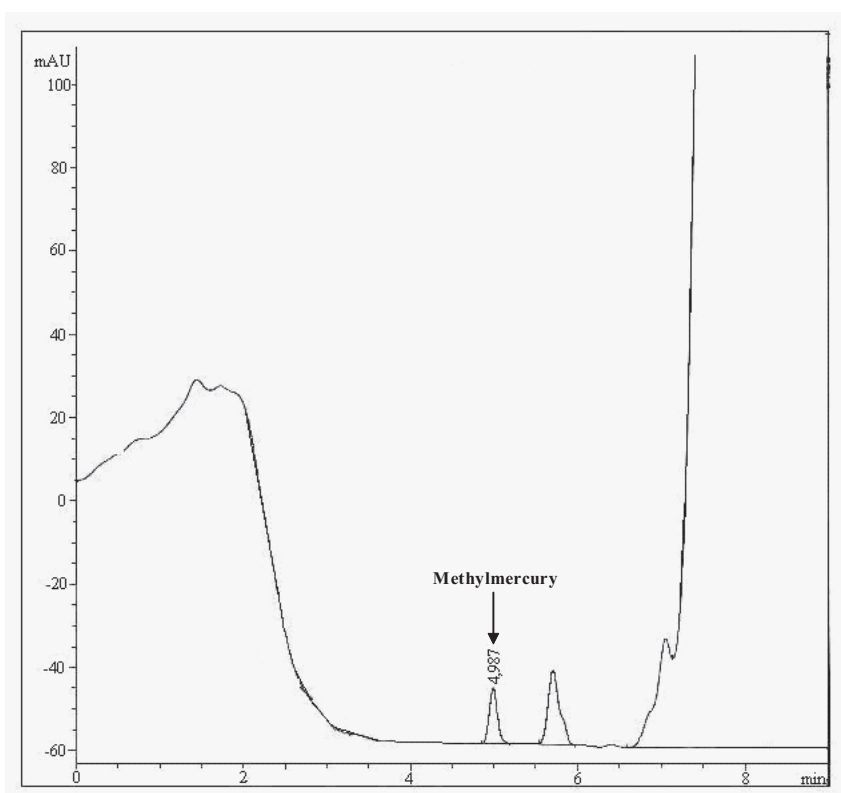
Figure 5. Chromatogram of the locality Frontera Peña—Orinoco contaminated with methylmercury standard of 50 ng.ml -1 , in a proportion 1:1. Retention time for MeHg = 4.99 minutes.
