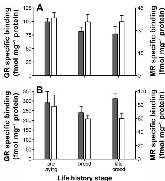
FIG. 4. Point sample analysis of glucocorticoid (GR; gray bars) and mineralocorticoid (MR; white bars) receptors in the (A) testes and (B) ovary of House Sparrows captured in Massachusetts at three life history stages ( n = 6 at each stage). Data represent means ( \pm SE) of specific binding of 10 nM [ ^3 H]CORT to House Sparrow cytosol, standardized by protein concentration. For more information, see Figure 1 caption.
