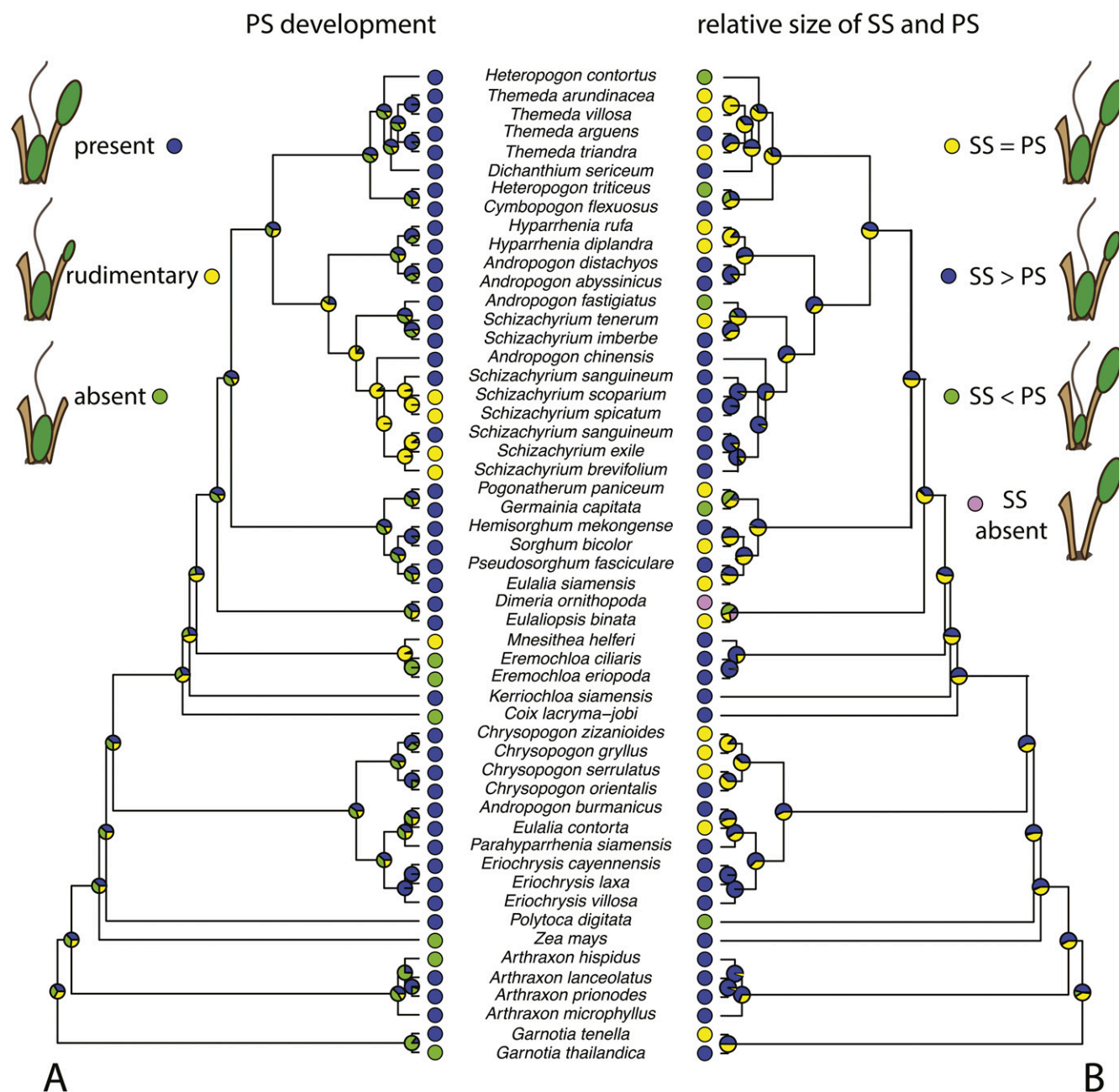
FIG. 3. Pedicellate spikelet (PS) development and relative size. A. the pedicellate spikelet may be present (blue circles), rudimentary (yellow), or absent (green). B. the sessile and pedicellate spikelets may be the same size (SS = PS, yellow), the sessile spikelet may be larger than the pedicellate spikelet (SS > PS, blue), the sessile spikelet may be smaller than the pedicellate spikelet (SS < PS, green), or the sessile spikelet may be absent (violet, only Dimeria ). The cartoon of each sessile-pedicellate pair shows, from left to right, the attached inflorescence internode (brown), the sessile spikelet (green) with its attached awn, the pedicel (brown), and the pedicellate spikelet.
