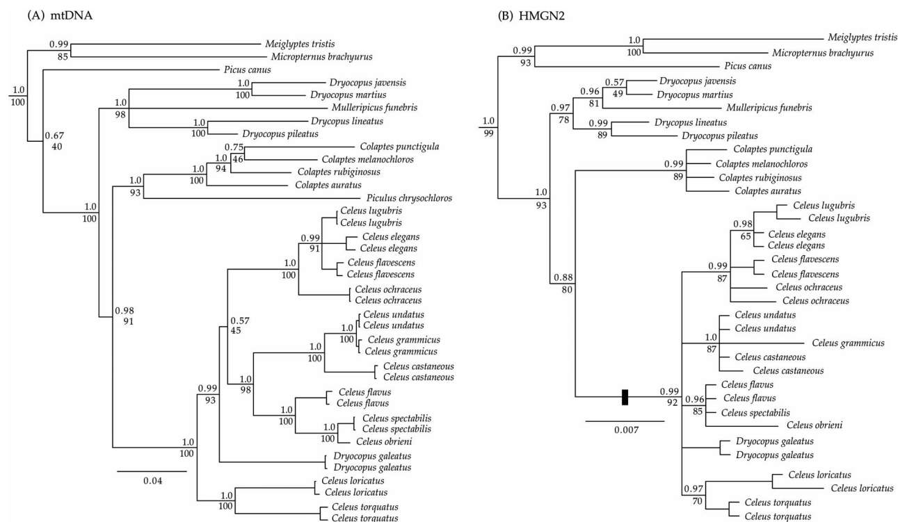
FIGURE 3. Phylogenetic relationships of the Helmeted Woodpecker ( Dryocopus galeatus ) inferred from (A) the combined mtDNA data matrix partitioned by codon position and (B) the HMGN2 nuclear locus. Bayesian posterior probabilities and maximum-likelihood bootstrap support values are indicated above and below each node, respectively.
