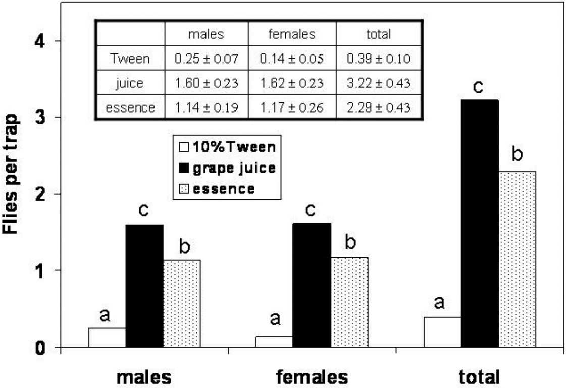
Fig. 1. Mean captures (± standard error) of irradiated Mexican fruit flies in traps baited with Frutibases grape juice and synthetic grape essence in a citrus orchard. Bars in the same sex with different letters are significantly different by Fishers Protected Least Significant Difference Test ( P < 0.05 ).
