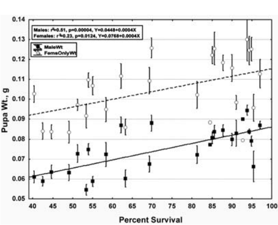
Fig. 3. Regression of male and female C. cactorum pupal weights on percent survival. Data from 1 container in which survival was < 22% has been deleted.
