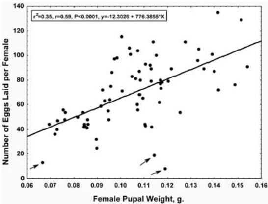
Fig. 4. Regression of number of eggs laid per female C. cactorum on pupal weight. Three outliers (arrows) representing fewer than 20 eggs are not included in the regression line.
