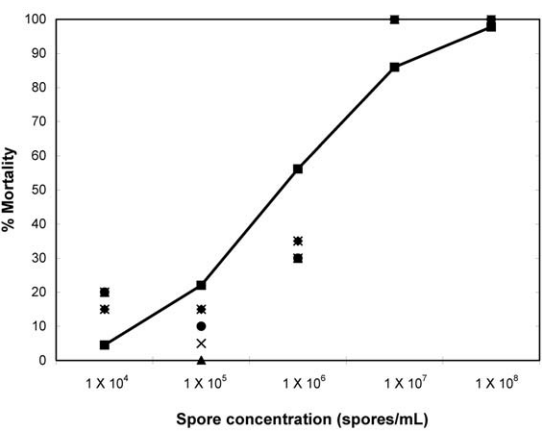
Fig. 3. Concentration-mortality curve for adults treated with Ifr AsCP after 192 h at 28 \pm 1^{\circ}\text{C} , under a 16L:8D photoperiod and \sim 100\% RH. The line was generated by Polo-Plus and the 5 means for each concentration are represented by the individual symbols, some of which are on top of each other.
