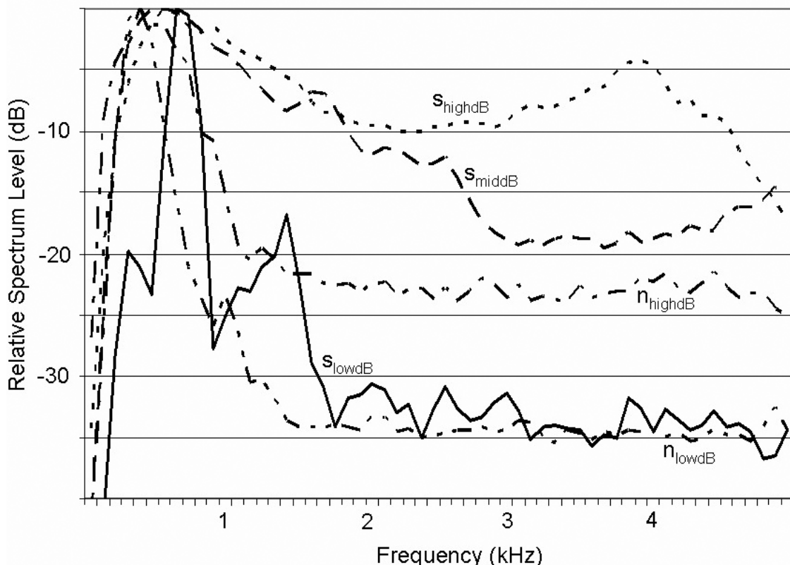
Fig. 1. Spectral profiles of insect-produced sound impulses, s_{highdB} , s_{middB} , and s_{lowdB} , compared with spectral profiles of wind-gust noise, n_{highdB} , and low-frequency background noise, n_{lowdB} , used in analyses to distinguish insect-produced sounds from background noise. The subscripts, highdB, middB, and lowdB, refer to the magnitudes of the relative spectrum levels of these profiles near 2.6 kHz, the midpoint of the 0.2-5 kHz range of frequencies analyzed. Spectrum level is relative to the maximum acceleration measured in the 0.2-5 kHz reference range.
