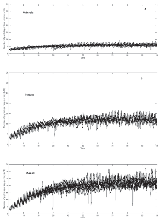
Fig. 4. Population dynamics with a stochastic carrying capacity for Diaphorina citri Kuwayama collected in 'Valencia' orange (a), 'Ponkan' mandarin (b), and 'Murcott' tangerine (c) trees in Taquaritinga, SP, Brazil.
