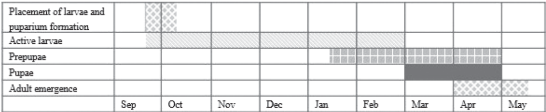
Fig. 2. Degree of progress, in months, toward transformation of Comadia redtenbacheri larvae weighing 0.30 g or more into adults.
