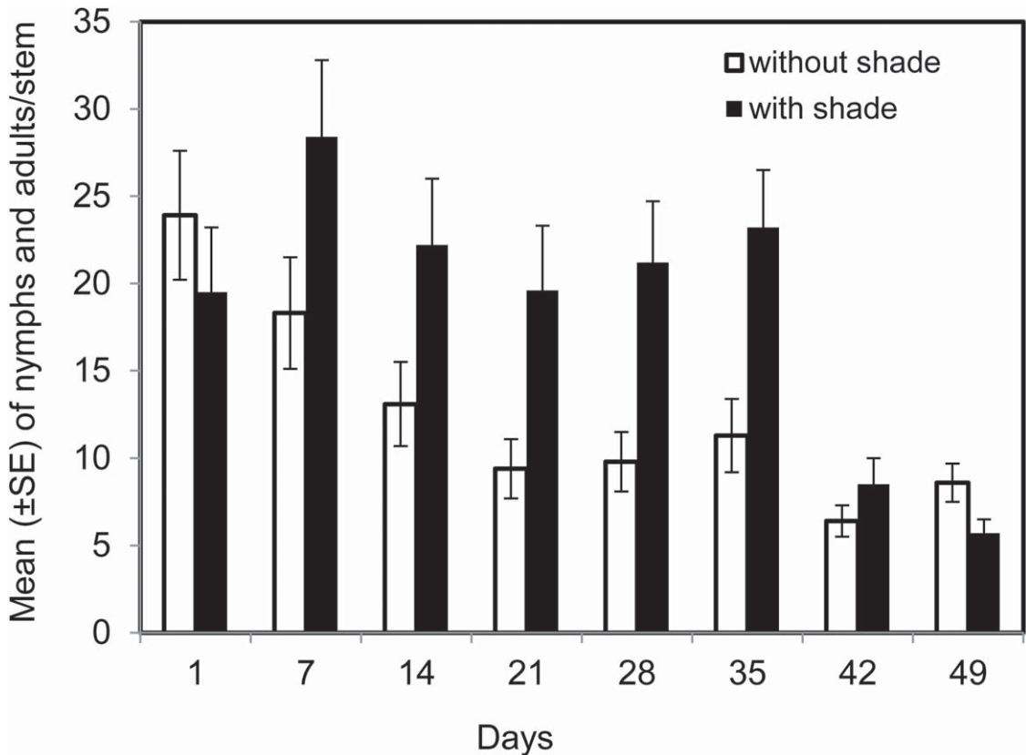
Fig. 2. Mean ( \pm SE) number of total Dalbulus quinquevittatus leafhoppers per stem on unshaded and shaded Tripsacum dactyloides . Day 1 is when nymphs first appeared.
