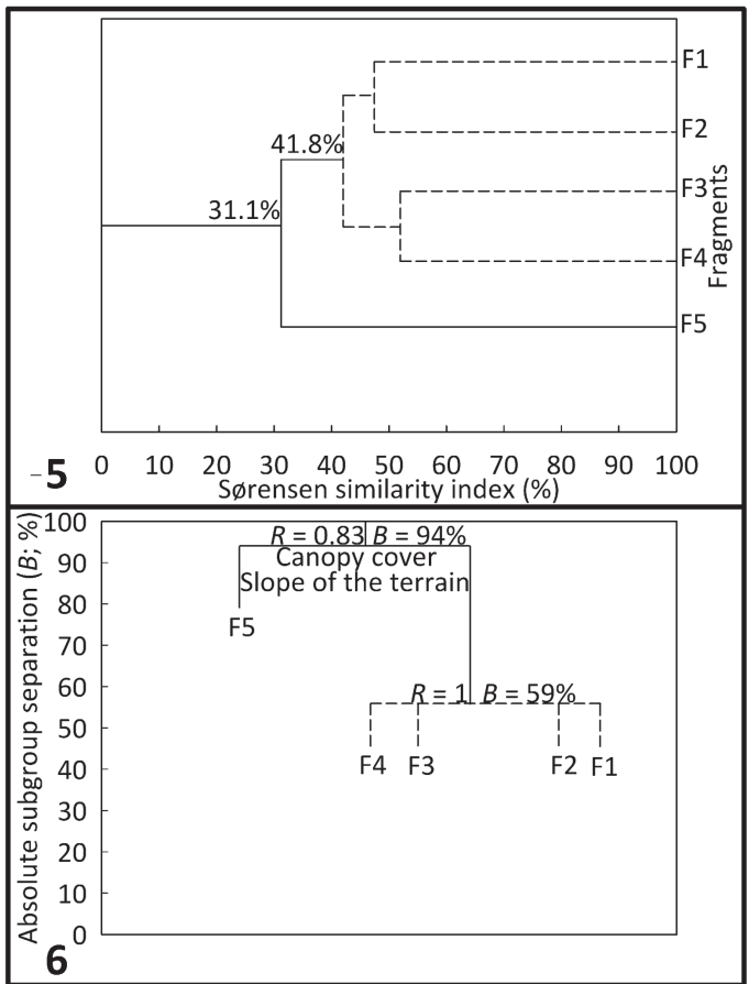
Figs. 5 and 6. Results from cluster and linkage tree analyses. Fig. 5. Dendrogram of hierarchical standardized clustering based on the Sørensen similarity index of the studied fragments. The cophenetic correlation coefficient of the cluster is 0.89. The dendrogram displays with continuous lines the divisions for which the SIMPROF test rejects the null hypothesis (where assemblages in that group have no further structure to explore) and with dashed lines the groups of assemblages not separated (at P < 0.05 ) by SIMPROF. Fig. 6. Linkage tree analysis (LINKTREE) showing divisive clustering of fragments (F1–F5) from species compositions constrained by inequalities on one or more environmental variables. Only binary partitions of uncorrelated environmental variables are shown in the cluster. The dendrogram displays with continuous lines the divisions for which the SIMPROF test rejects the null hypothesis (where assemblages in that group have no further structure to explore) and with dashed lines the groups of assemblages not separated (at P < 0.05 ) by SIMPROF.
