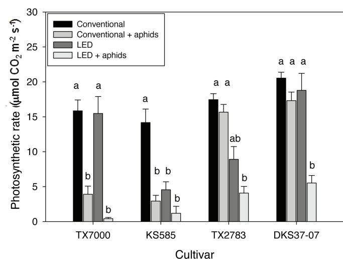
Fig. 5. Mean \pm SE photosynthetic rates ( \mu\text{mol CO}_2 \text{ m}^{-2} \text{ s}^{-1} ) of resistant (TX-7000 and KS-585) and susceptible (TX-2783 and DKS-37-07) sorghum cultivars grown under either conventional or light-emitting diodes. All plants were measured at 15 d after infestation with sugarcane aphids. Bars with different letters are significantly different (Kruskal-Wallis ANOVA, df = 3 ; H > 27.14 ; P < 0.01 ).
