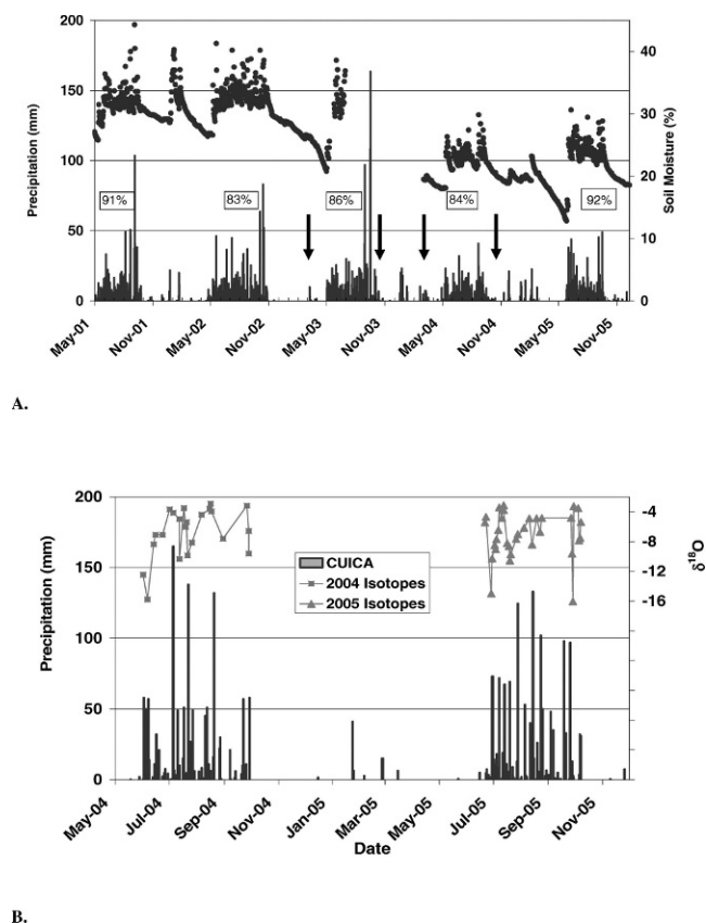
FIGURE 6. (A) Daily precipitation (bars) and volumetric soil moisture (dots) as measured at the Nevado de Colima site from 2001 to 2005 (see Biondi et al., 2005, for details). Percentages indicate the monsoon precipitation (June to October) with respect to the total precipitation for the water year (June to May). Arrows indicate the timing of the isotopic sampling events at the Nevado de Colima study area. (B) Stable isotopic composition of monsoon precipitation events, and precipitation amounts, as collected in Colima City during the monsoon, 2004–2005.
