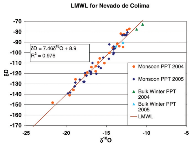
FIGURE 4. Isotopic ratios of samples collected from individual storms in 2004 and 2005 at the Universidad de Colima ("Centro Universitario de Investigaciones en Ciencias del Ambiente"; elevation \sim 400 m), and scaled for the elevation difference between that site and the study area at Nevado de Colima ( \sim 3800 m). Also plotted are bulk precipitation samples from the study area. A Local Meteoric Water Line (LMWL) was obtained by fitting a linear regression equation to the stable isotope data.
