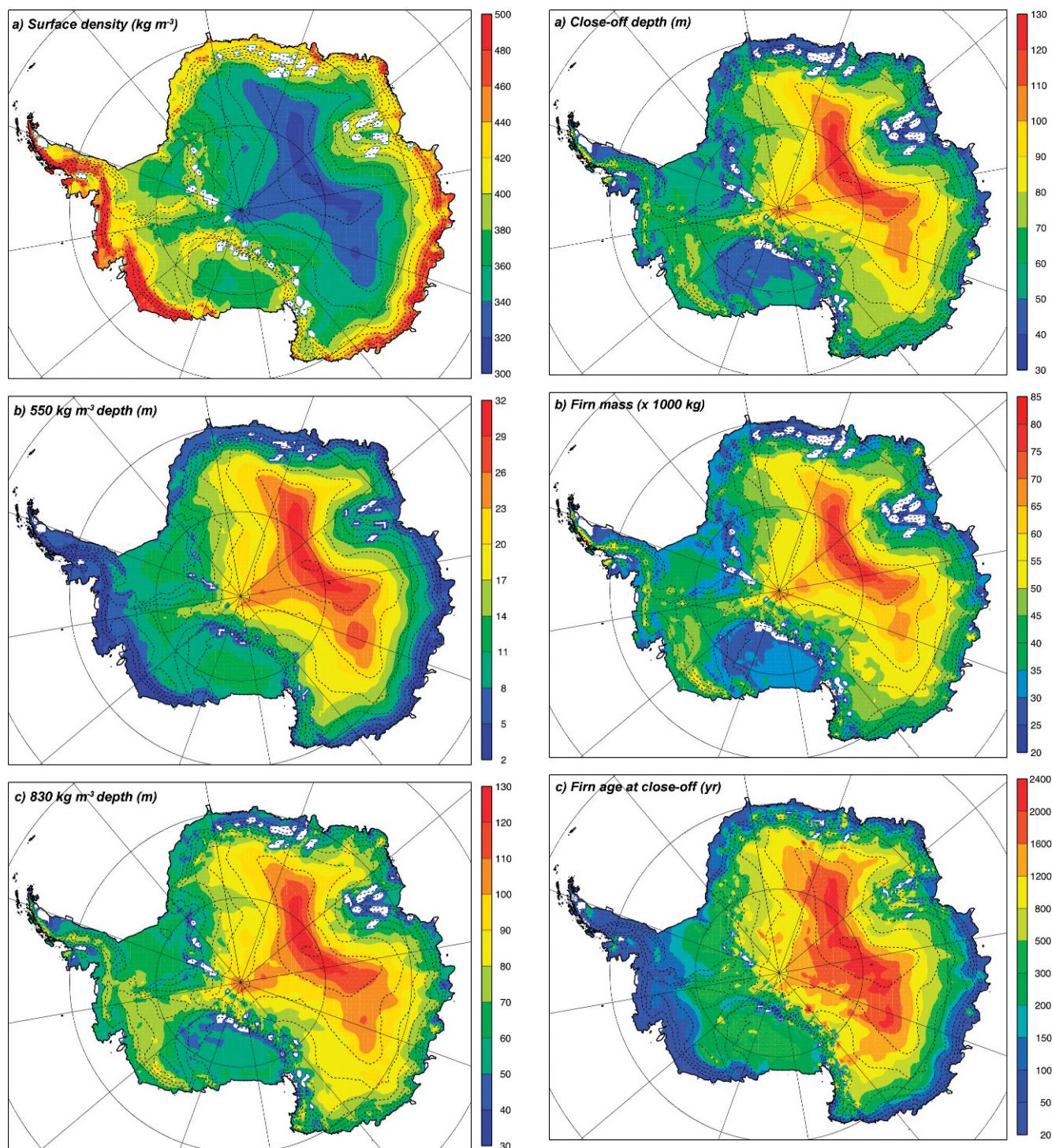
FIGURE 7. Modeled depth of pore close-off (a), firn mass above pore close-off (b), and age of firn at pore close-off (c).
