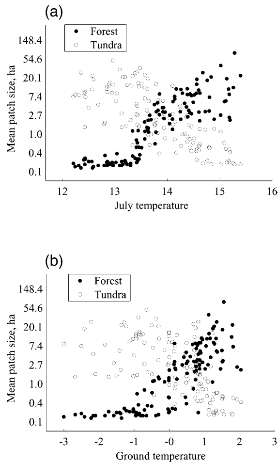
FIGURE 4. The mean patch size of the forest and tundra patches in relation to (a) mean July temperature; (b) mean ground temperature. The observations are the mean values of the lowland 25 \times 25 km grid cells seen in Figure 7c. The y-axes are in logarithmic scale.
