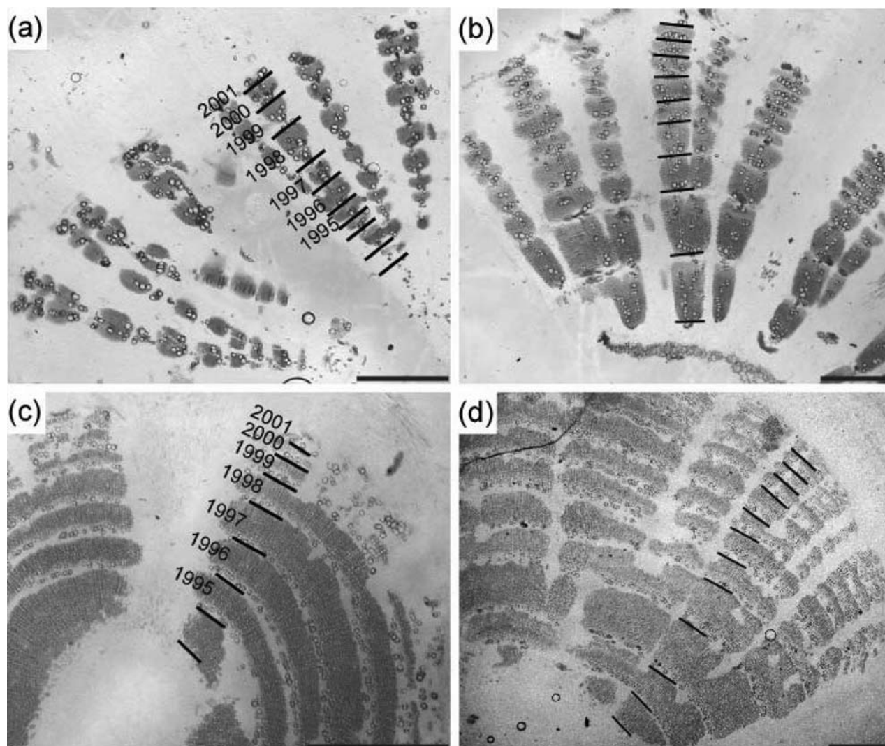
FIGURE 2. Patterns of growth rings in the secondary root xylem of Cirsium spinosissimum (a, b) and Pedicularis recutita (c, d). The samples in (a) and (c) were collected in the center of the snowbank whereas the samples in (b) and (d) were obtained from the periphery of the snowbank. The markers along the xylem radii denote transition from latewood of the previous growing period to earlywood of the following one. The distance between consecutive markers represents the width of the enclosed growth ring. The horizontal bars indicate 1 mm.
