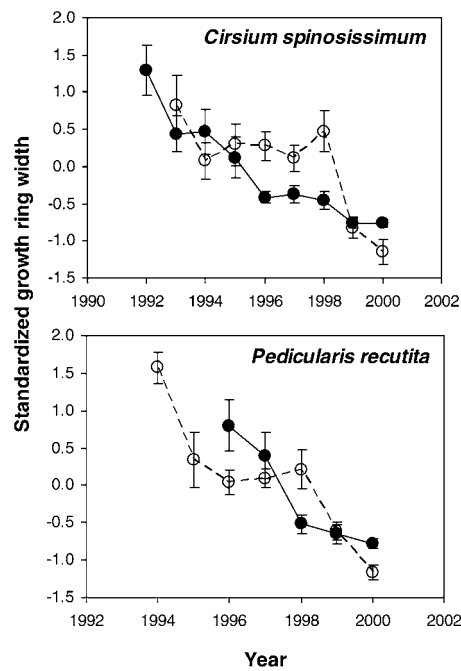
FIGURE 3. Standardized growth ring widths (mean \pm 1 S.E.) in the secondary xylem of Cirsium spinosissimum and Pedicularis recutita in relation to the calendar year. Open circles/dashed lines indicate samples obtained from the snowbank center; filled circles/solid lines denote samples collected from the peripheral zone. See text for further information.
