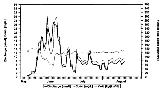
Discharge, conc., and yield of dissolved solids; Latnjavagge, Outlet (2001 field season)
