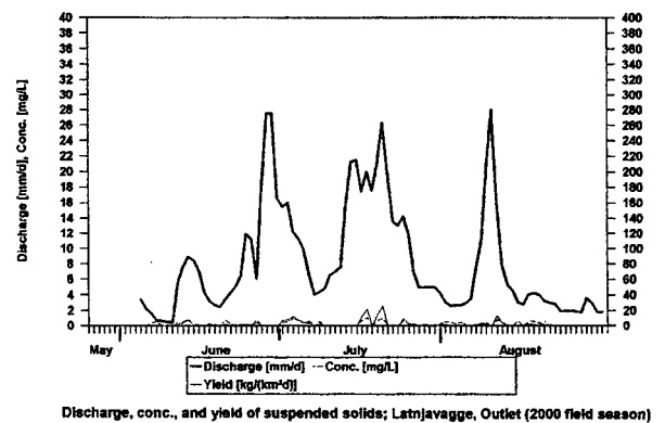
Discharge, conc., and yield of suspended solids; Latnjavagge, Outlet (2000 field season)
