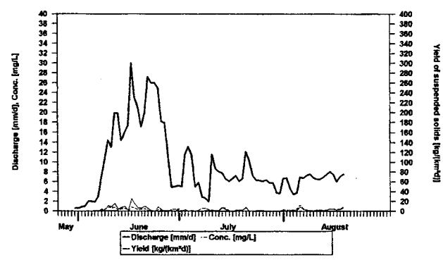
Discharge, conc., and yield of suspended solids; Latnjavagge, Outlet (2001 field season)
