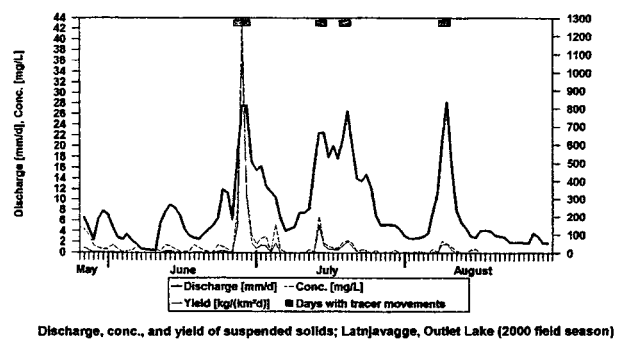
Discharge, conc., and yield of suspended solids; Latnjavagge, Outlet Lake (2000 field season)
