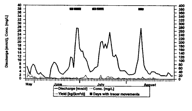
FIGURE 5. Daily specific runoffs, concentrations, and yields of suspended sediments; Outlet Latnjavagge, outlet lake and inlet lake Latnjajaure: (a) 2000 field season, (b) 2001 field season.
