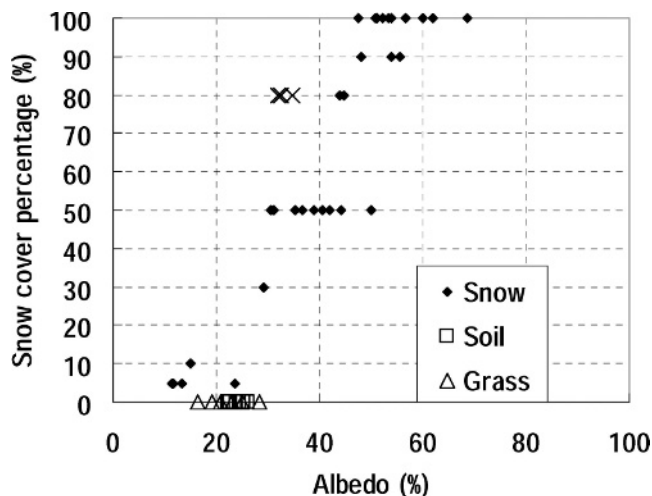
FIGURE 11. Relationship between albedo and snow cover percentage. Crosses indicate observation points located in the bottom of the valley with snow covered slopes.
