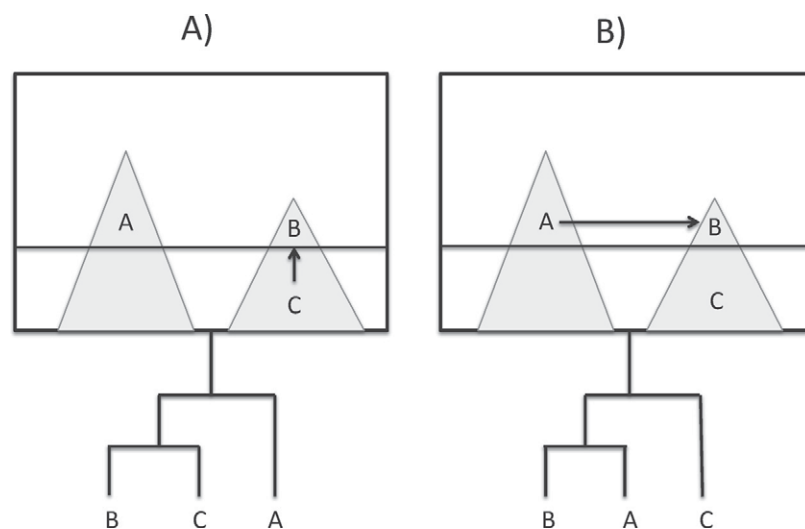
FIGURE 6. (a) Expected phylogenetic relationship for an adaptive radiation origin of a summit speciation event. (b) Expected phylogenetic relationship for a geographic speciation (vicariant) origin of a summit speciation event.
