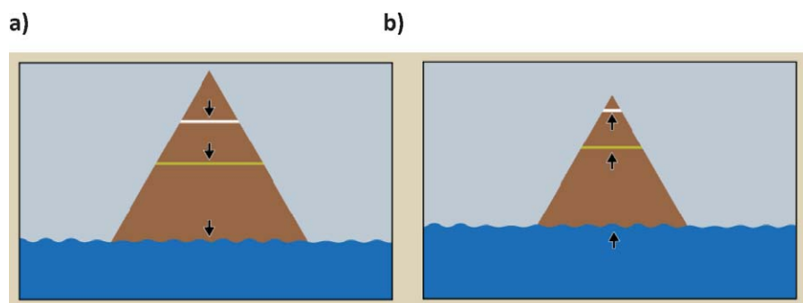
FIGURE 4. (a) Downward retreat of the snowline, timberline, and sea level after the onset of a glaciation period, and (b) upward retreat of the snowline, timberline, and sea level after the onset of an interglacial period.
