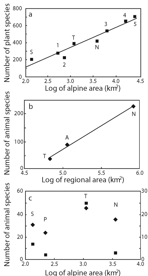
FIGURE 3. The relationship between land area and the diversity of species for (a) alpine vascular plants (S = Snowy Mountains, T = Tasmania, N = New Guinea, 1 = Afro-alpine, 2 = Hokkaido, 3 = Sierra Nevada [U.S.A.], 4 = Swiss Alps, and 5 = Southern Alps [New Zealand]), (b) regional vertebrate fauna (T = Tasmania, A = Australian mainland, N = New Guinea), and (c) alpine vertebrate fauna (diamonds left axis) and alpine fauna as a percentage of the regional fauna (squares right axis) (S = Snowy Mountains, P = PNG only, T = Tasmania, N = whole of New Guinea).
