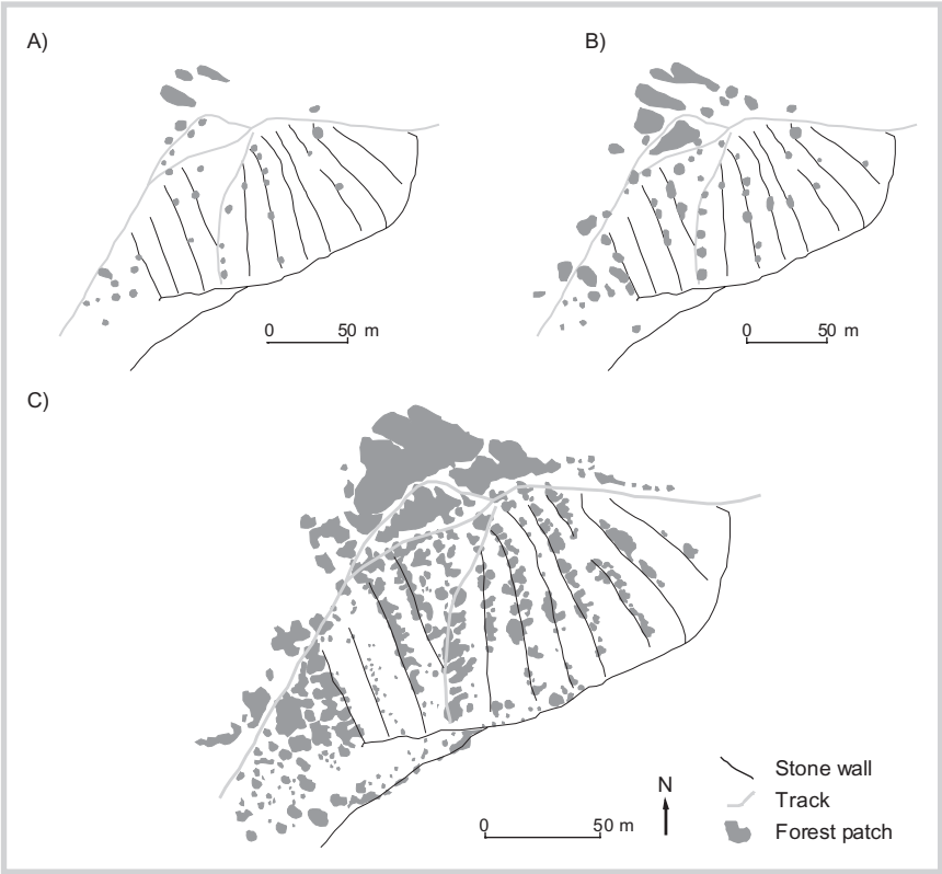
FIGURE 3 Development of forested area on a terraced site in the study area: (A) 1957, (B) 1977, and (C) 1996.
