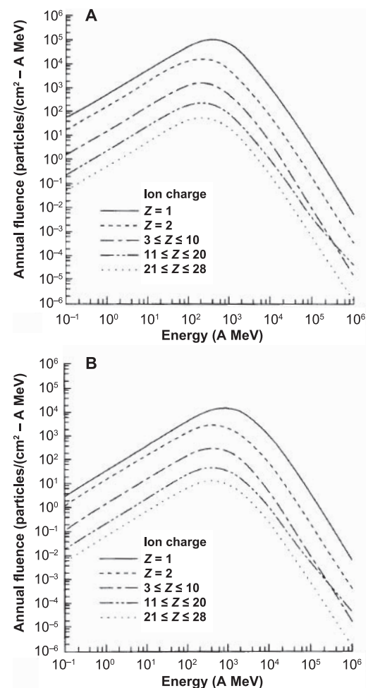
FIG. 2. Differential annual fluence spectra. Panel A: GCR ion fluence for 1977 solar minimum. Panel B: GCR ion fluence for 1981 solar maximum. Here energy has been multiplied by atomic number, A , rather than expressed as E/n . Note overall reduction in fluence but increase in energy of fluence maximum for solar max. Reproduced and used with permission from Fig. 1 of Wilson et al. (37).
