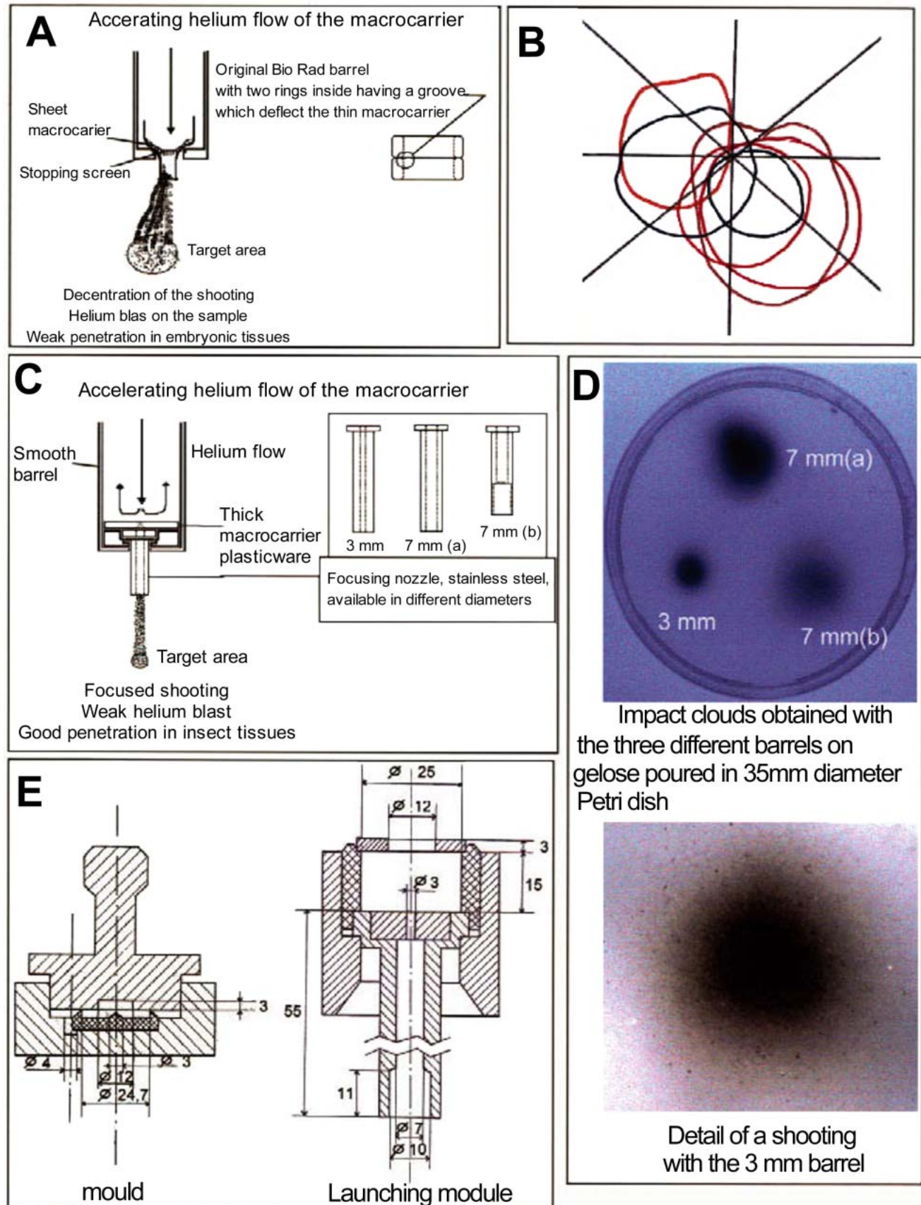
Figure 1. Mechanical modifications on the Bio Rad PDS/1000 He biolistic device shooting module. A: Schematic illustration of the problems encountered with the original shooting module. B: Decentering of the shootings with the original shooting module. C: Schematic illustration of our mechanical modifications. D: Focusing the shootings with our shooting module. E: Plan of our macrocarrier mould (left) and the shooting module (right).
